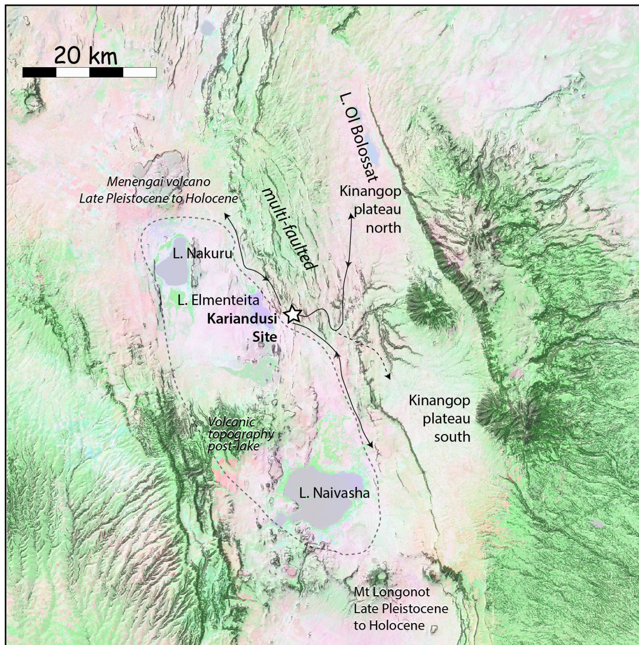
Figure 8. Morphology of the region including Lakes Nakuru, Elmenteita, Naivasha and Bolossat. Slopes greater than 15° are indicated by grey shading, and would have restricted movements of large animals to well defined areas and restricted pathways that converge on the Kariandusi location. Lakes Nakuru, Elmenteita and possibly Naivasha were joined to form a single lake, shown by the blue area enclosed by a dashed line, during periods of high lake level. Some earlier features (that pre-date the Kariandusi site) have been masked by later volcanism between Elmenteita and Naivasha and around Menengai volcano and Mt. Longonot (see Figure 9)
