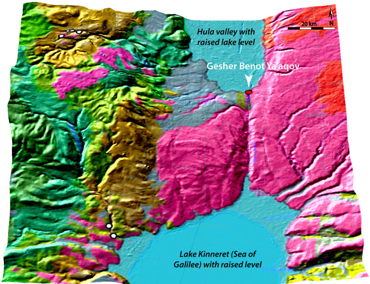
Figure 15. Oblique 3D view of the region around Gesher Banot Ya'acov in relation to geology and topography at the time of its occupation. The image is based on etm+ legacy data. Topography from SRTM v4.1 data with a vertical exaggeration of ~8. Colour coding of geology as in Figure 14. Note the restricted corridor between the expanded Lake Hula to the north and the steep-sided Upper Jordan valley to the south. This forms a natural ambush for trapping large mammals moving between the grazing lands west of the Rift valley and the Golan Heights. After Devès et al. 2014.
