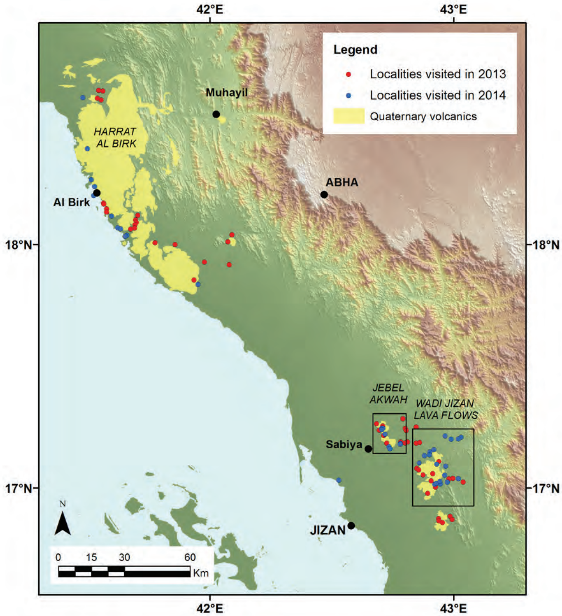
Figure 7.1: Map of locations showing localities visited by DISPERSE in 2013 and 2014 in Jizan and Asir regions. Elevation data © CGIAR-CSI SRTM 90m v4.1 database.
