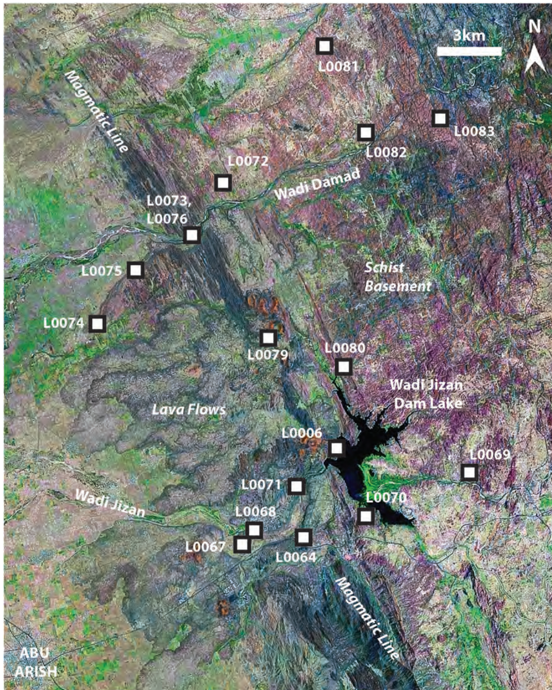
Figure 7.6: Locations of sites visited around the Abu Arish lava flows and upper coastal plain. The extensive lava flows are visible to the West of Magmatic Line and the Wadi Jizan Dam Lake, the latter in the lower centre of the figure. To the North and East of the lake, the exposed schistic basement is visible as a purple colour. Satellite Imagery © USGS Landsat ETM+ 2000 Geocover Mosaics.
