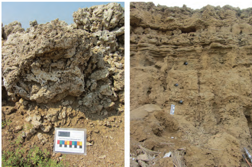
Figure 7.20: a) A coral terrace towards the North of the locality, dissected by bulldozing. Scale is 10 cm b) Section through marine deposits in main quarry sampled for OSL dating. Scale is 30 cm. Photos: R. Inglis.
