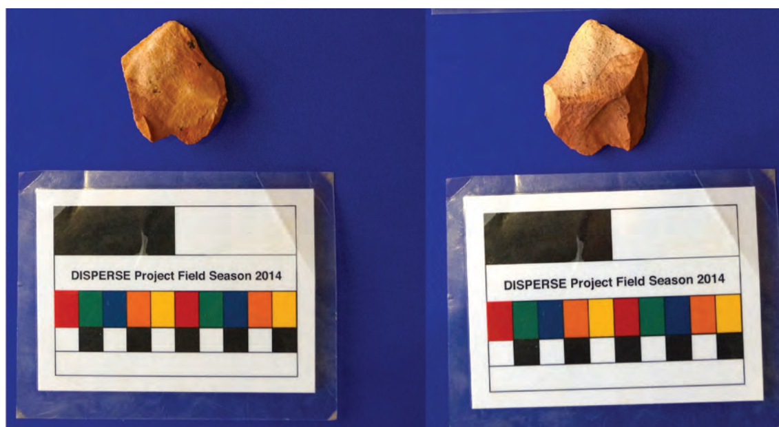
Figure 7.8: Discoidal flake from section under lava at L0064. Photo: A. Shuttleworth.
