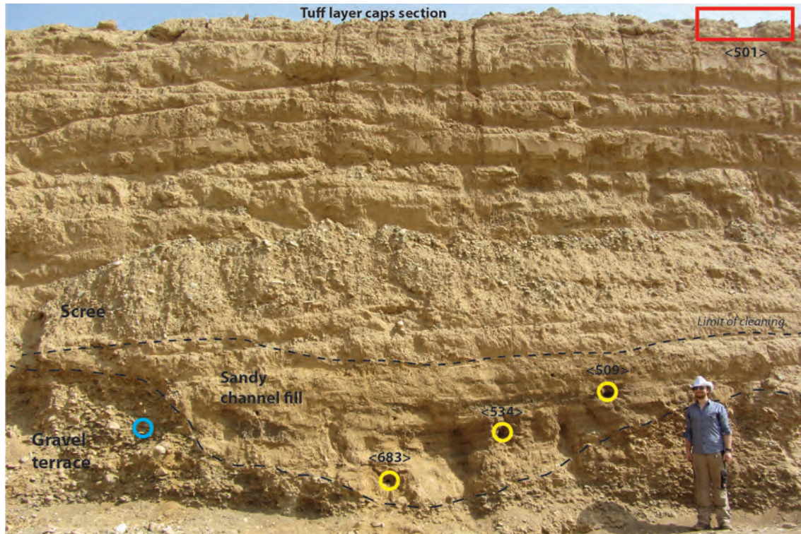
Figure 7.4: Quarry section at L0020, near Wadi Sabiya. The section shows a cross-section through a wadi channel, with gravel terraces incised by a channel, later filled by a sandy channel fill. A worked clast (Figure 7.5) was recovered from the left hand gravel terrace (blue circle). Dating samples were taken from the channel fill for OSL (yellow circles), and a sample of tuff was taken from the top of the section (red rectangle). Photo: R. Inglis.
