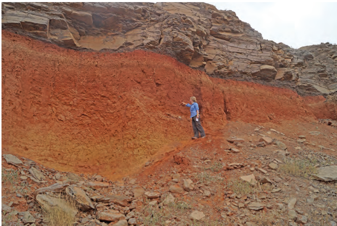
Figure 7.7: Section through fine-grained floodplain sediments under lava flow at L0064. Figure is indicating where discoidal flake was found embedded in section. Photo: G. Bailey.
