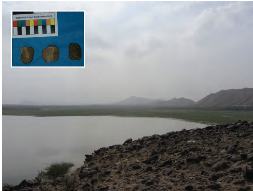
Figure 7.9: A view from L0006 looking East across Wadi Jizan Dam Lake. Inset: MSA prepared core flakes located at L0006. Photos: A. Sinclair.
