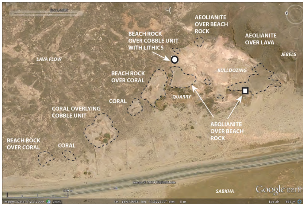
Figure 7.19: Aerial view of Dhahaban Quarry, L0034, showing key geomorphological units at the locality. The circle indicates location of stratified lithics. The square indicates location of sampling of beach and shallow marine deposits for OSL dating. Image © DigitalGlobe accessed through Google Earth. Imagery Date 21/9/2009
