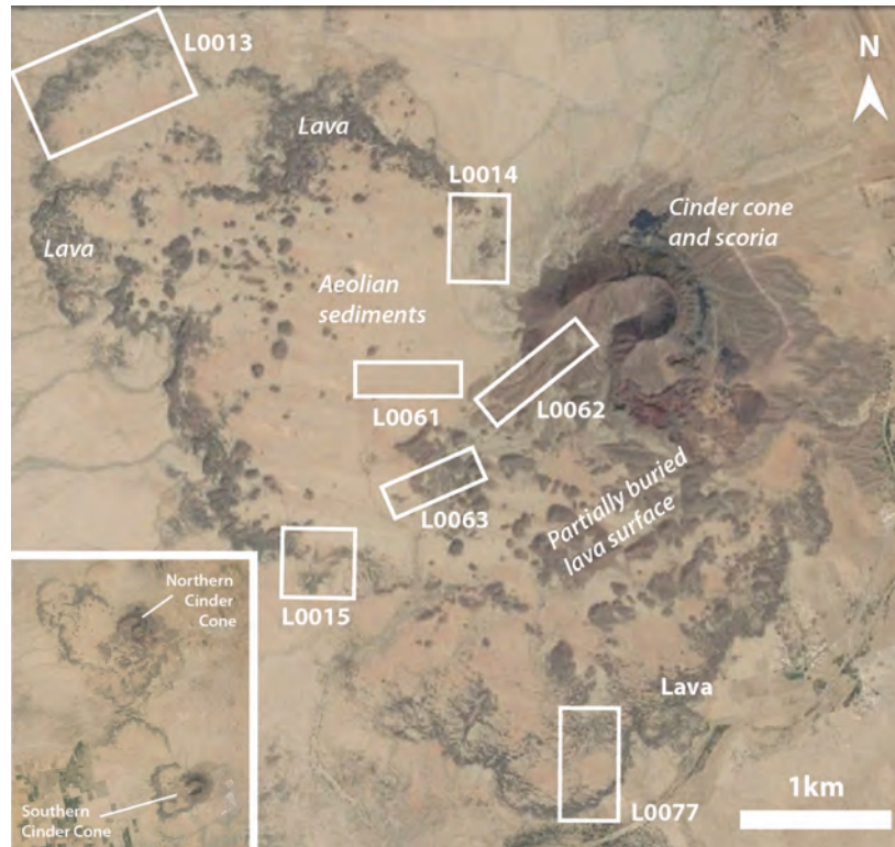
Figure 7.2: Map showing northern Jebel Akwah cinder cone, and the localities visited in 2013 and 2014 and major geomorphological features. L0061-63 and L0077 were visited in 2014. Inset shows overview of Jebel Akwah. Satellite imagery © DigitalGlobe 2014, accessed through Google Earth. Imagery Date 3/6/2014.
